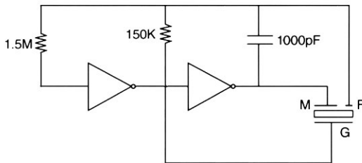
Reference Circuit
